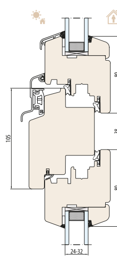
SYSTEM NATURO 68 Querholz 105 mm
