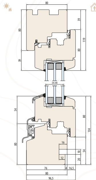
SYSTEM NATURO 80 Innere Fensterbankfräsung
