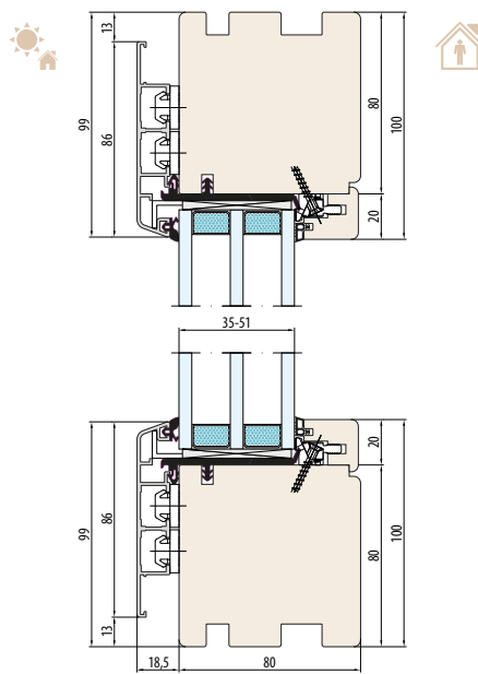
SYSTEM NATURO 80 ALU-Fix GEMINI CLASSIC
