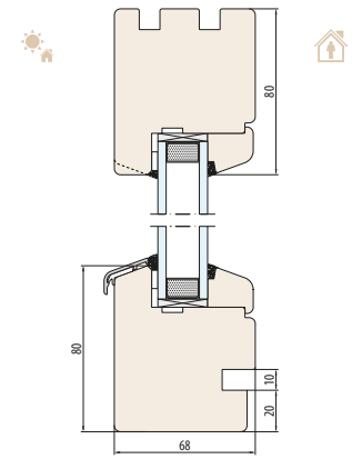
SYSTEM NATURO 68-Fix Innere Fensterbankfräsung
